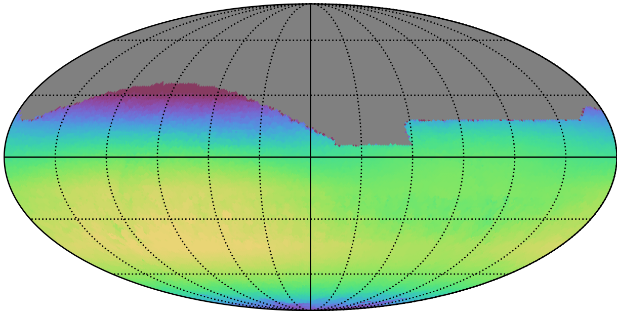
too_elab_r8_d3_giz_v3.4_10yrs All sky i band: Max skyBrightness
