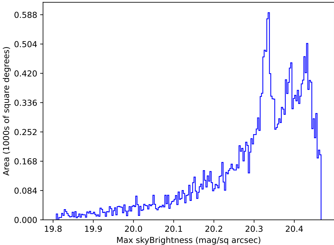
too_elab_r8_d3_giz_v3.4_10yrs All sky i band: Max skyBrightness
