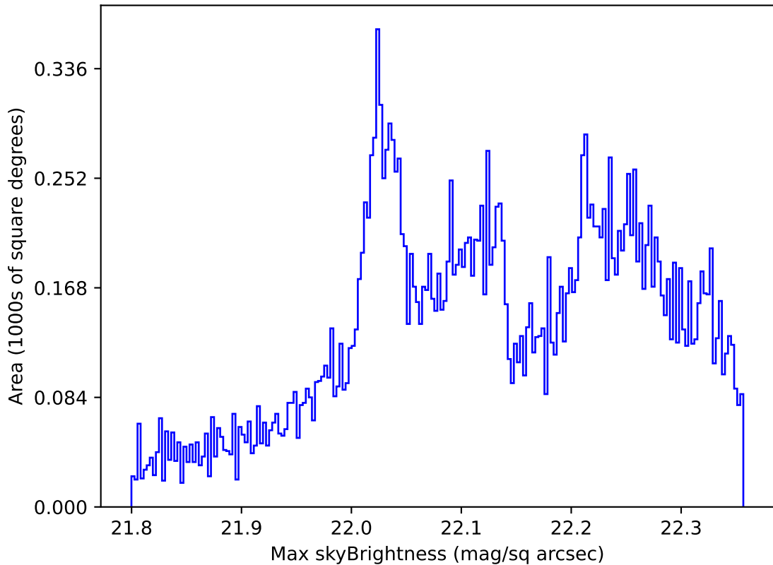
too_elab_r8_d3_giz_v3.4_10yrs All sky g band: Max skyBrightness
