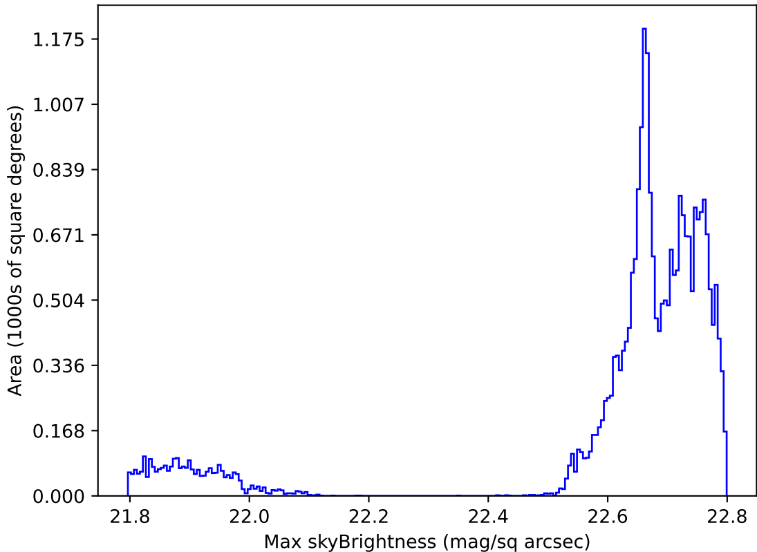
too_elab_r8_d3_giz_v3.4_10yrs All sky all bands: Max skyBrightness
