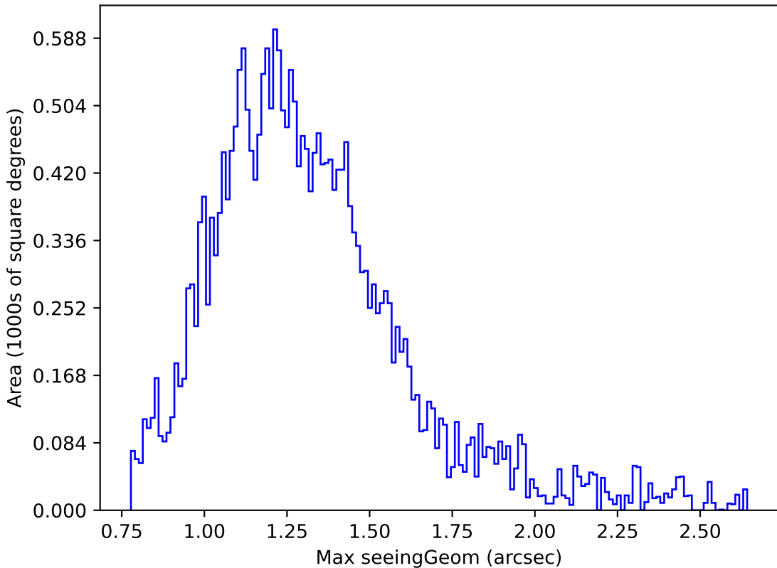
too_elab_r8_d3_giz_v3.4_10yrs Yr 1 z band: Max seeingGeom
