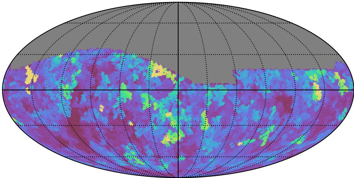
too_elab_r8_d3_giz_v3.4_10yrs Yr 1 z band: Max seeingEff
