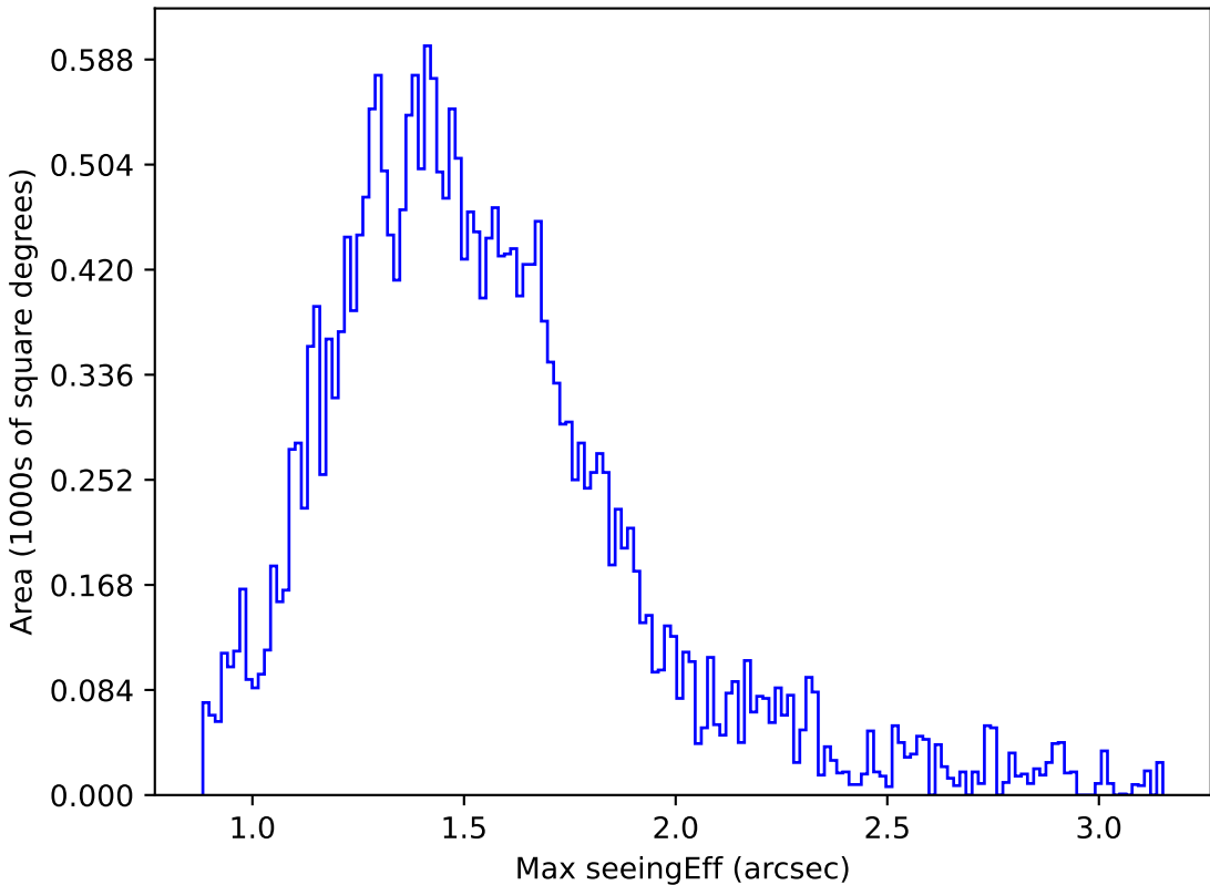
too_elab_r8_d3_giz_v3.4_10yrs Yr 1 z band: Max seeingEff
