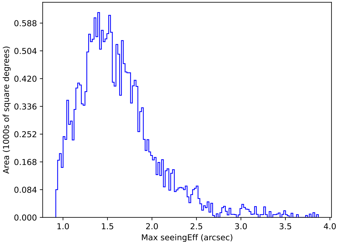
too_elab_r8_d3_giz_v3.4_10yrs Yr 1 u band: Max seeingEff
