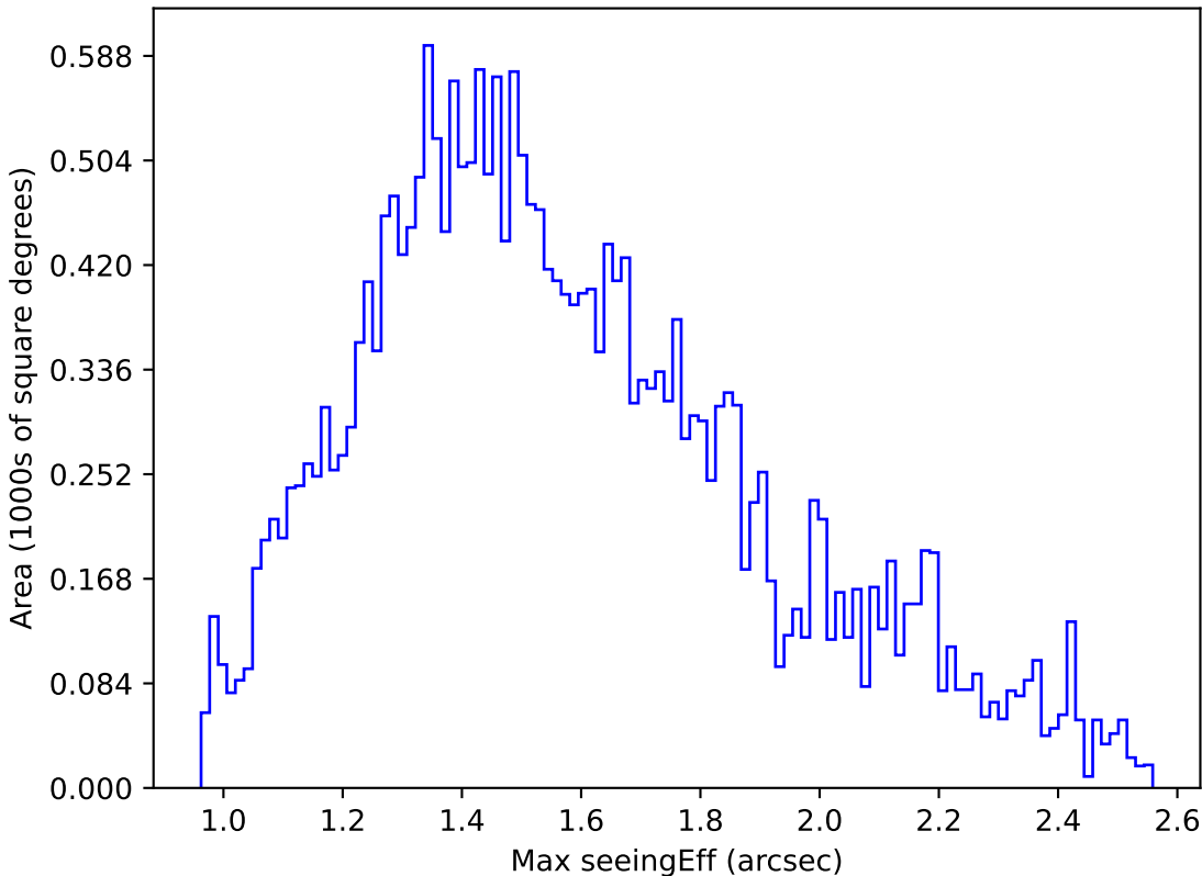
too_elab_r8_d3_giz_v3.4_10yrs Yr 1 r band: Max seeingEff
