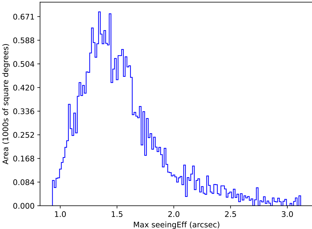
too_elab_r8_d3_giz_v3.4_10yrs Yr 1 g band: Max seeingEff
