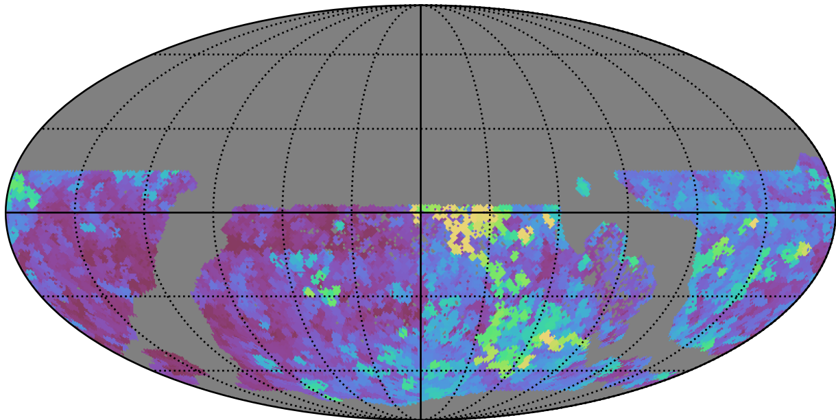
too_elab_r8_d3_giz_v3.4_10yrs WFD y band: Max seeingEff
