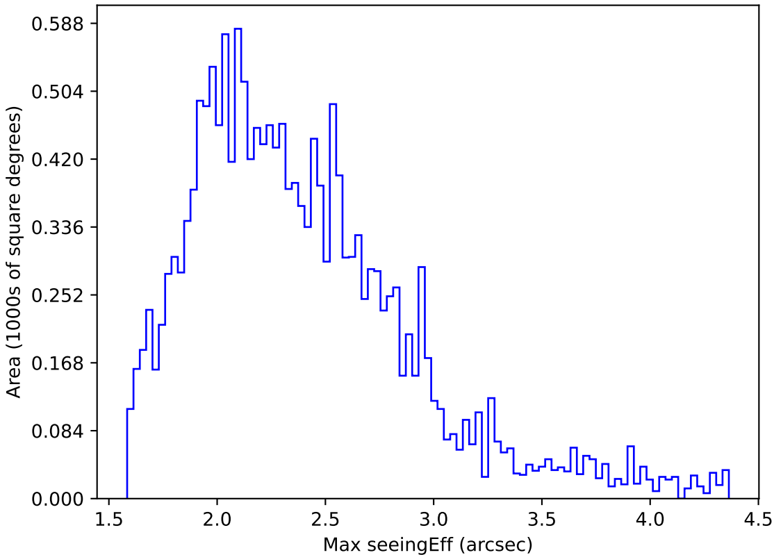
too_elab_r8_d3_giz_v3.4_10yrs WFD y band: Max seeingEff
