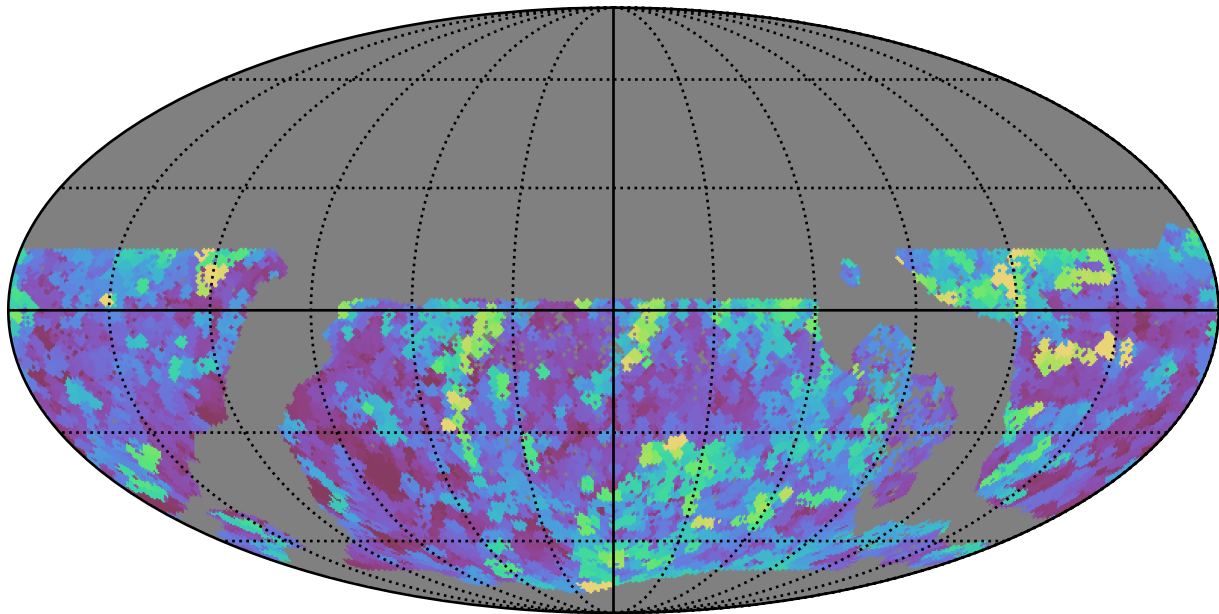
too_elab_r8_d3_giz_v3.4_10yrs WFD r band: Max seeingEff
