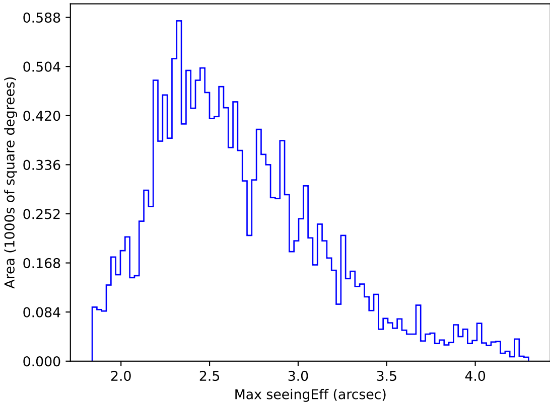
too_elab_r8_d3_giz_v3.4_10yrs WFD r band: Max seeingEff
