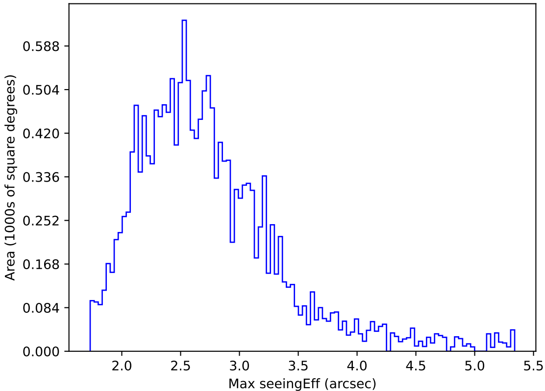
too_elab_r8_d3_giz_v3.4_10yrs WFD i band: Max seeingEff
