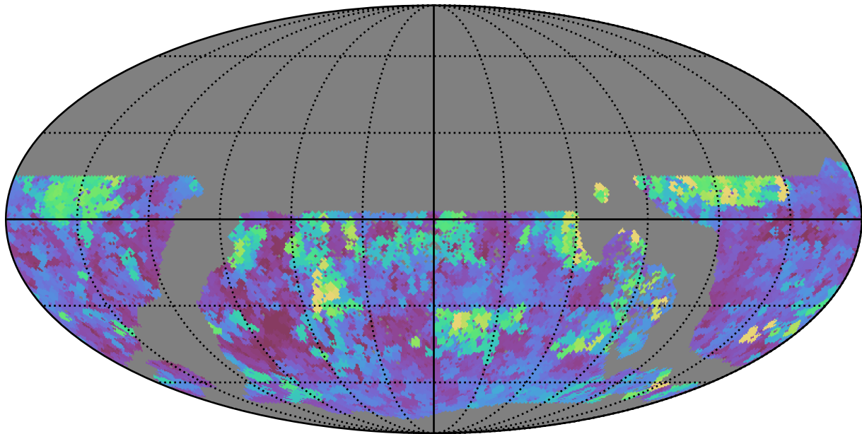
too_elab_r8_d3_giz_v3.4_10yrs WFD g band: Max seeingEff
