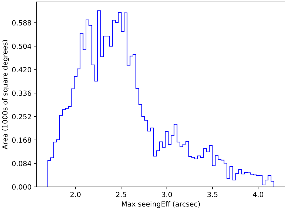
too_elab_r8_d3_giz_v3.4_10yrs WFD g band: Max seeingEff
