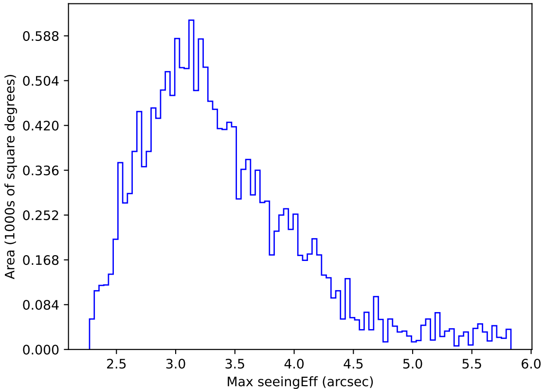
too_elab_r8_d3_giz_v3.4_10yrs WFD all bands: Max seeingEff
