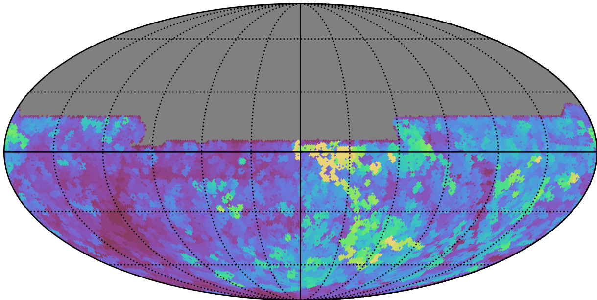
too_elab_r8_d3_giz_v3.4_10yrs All sky y band: Max seeingEff
