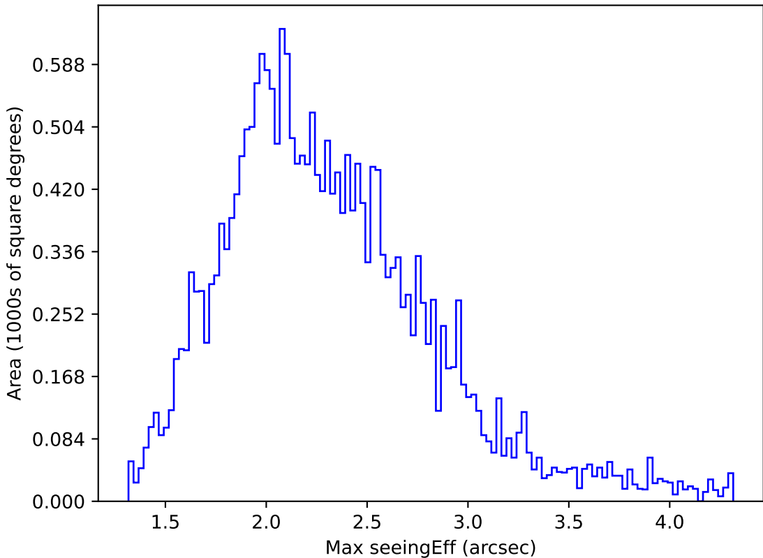
too_elab_r8_d3_giz_v3.4_10yrs All sky y band: Max seeingEff
