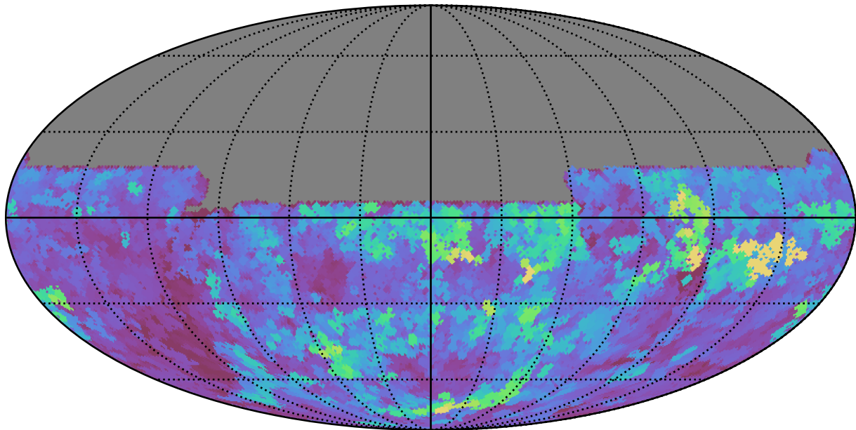
too_elab_r8_d3_giz_v3.4_10yrs All sky u band: Max seeingEff
