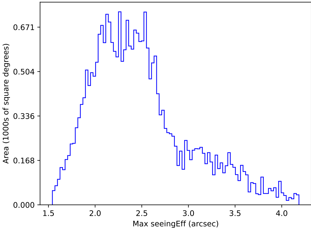
too_elab_r8_d3_giz_v3.4_10yrs All sky g band: Max seeingEff
