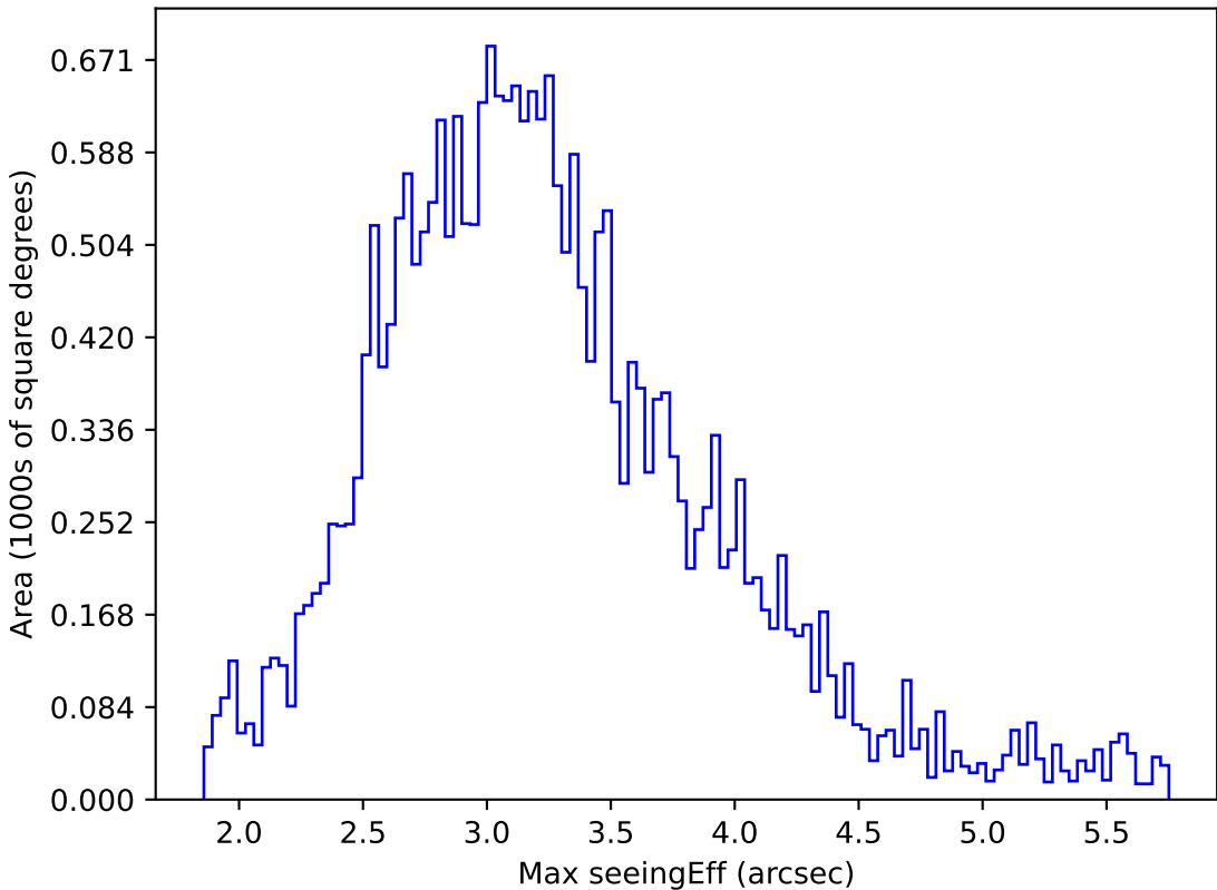
too_elab_r8_d3_giz_v3.4_10yrs All sky all bands: Max seeingEff
