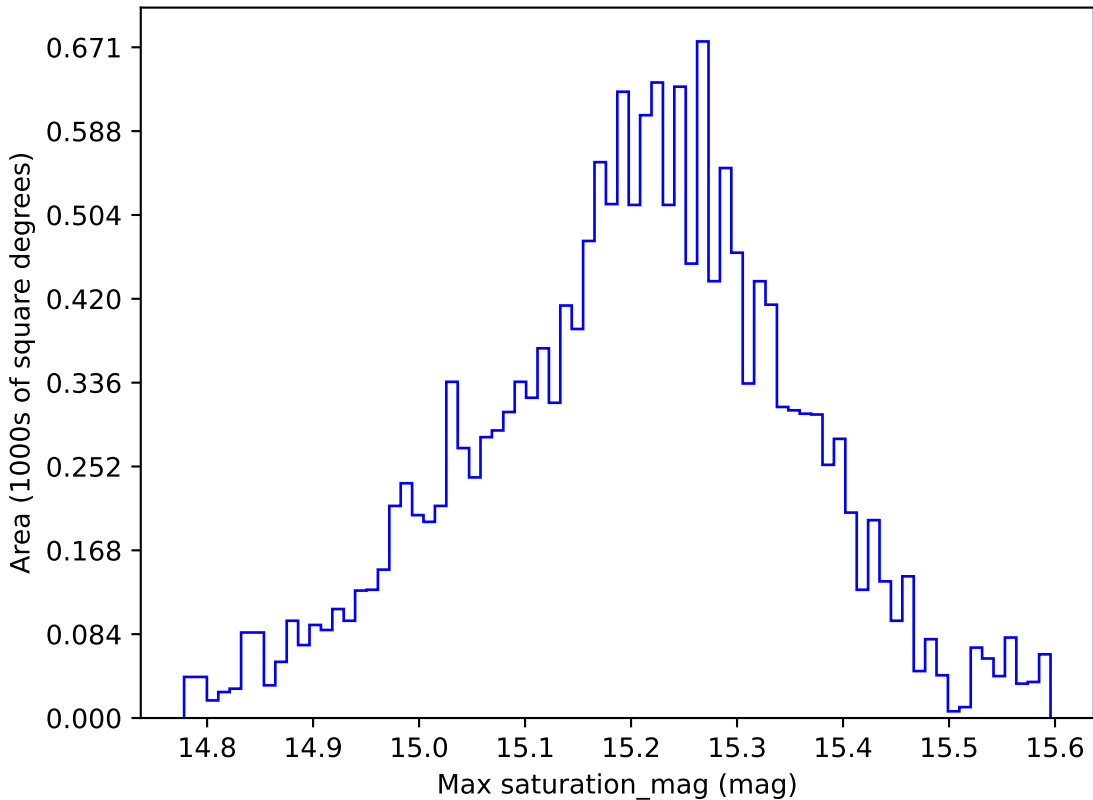
too_elab_r8_d3_giz_v3.4_10yrs WFD z band: Max saturation_mag
