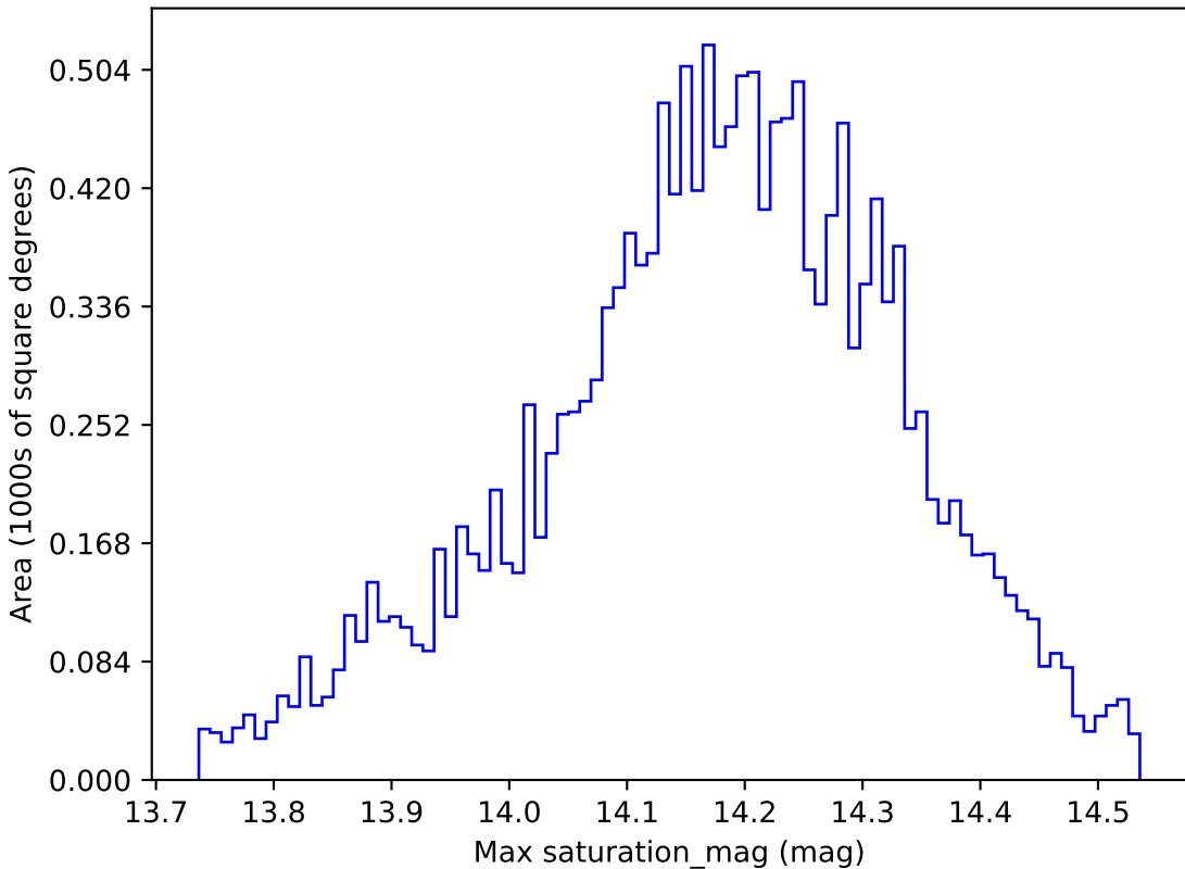
too_elab_r8_d3_giz_v3.4_10yrs WFD y band: Max saturation_mag
