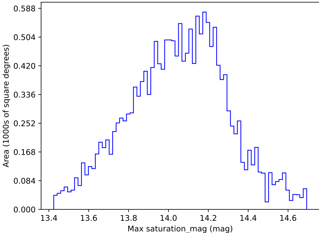
too_elab_r8_d3_giz_v3.4_10yrs WFD u band: Max saturation_mag
