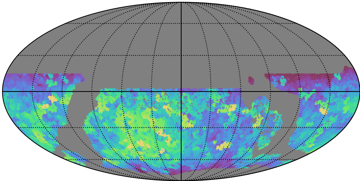
too_elab_r8_d3_giz_v3.4_10yrs WFD r band: Max saturation_mag
