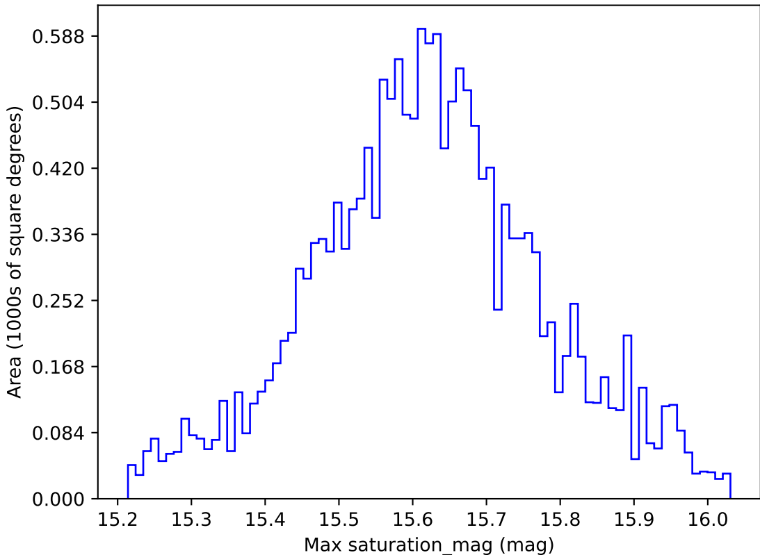
too_elab_r8_d3_giz_v3.4_10yrs WFD i band: Max saturation_mag
