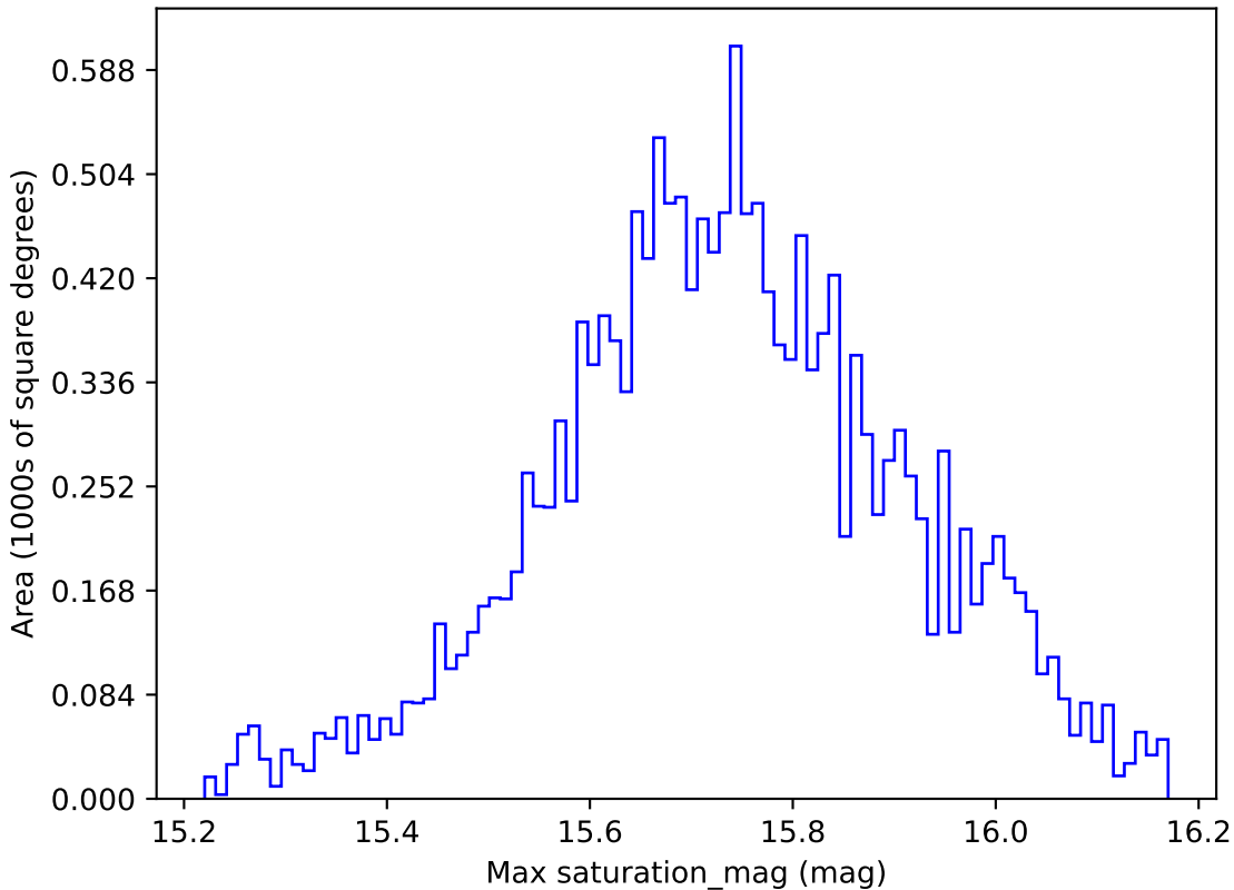
too_elab_r8_d3_giz_v3.4_10yrs WFD g band: Max saturation_mag
