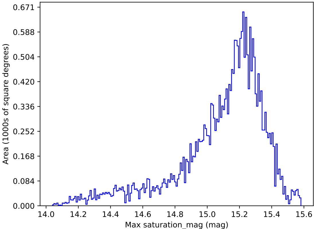
too_elab_r8_d3_giz_v3.4_10yrs All sky z band: Max saturation_mag
