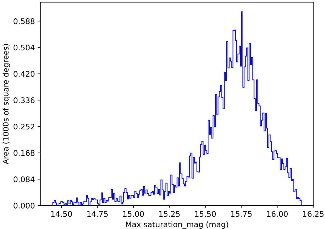
too_elab_r8_d3_giz_v3.4_10yrs All sky r band: Max saturation_mag
