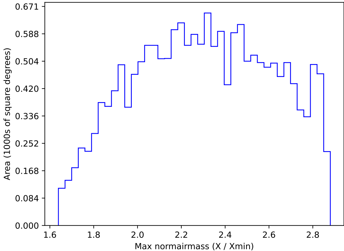
too_elab_r8_d3_giz_v3.4_10yrs WFD z band: Max normairmass
