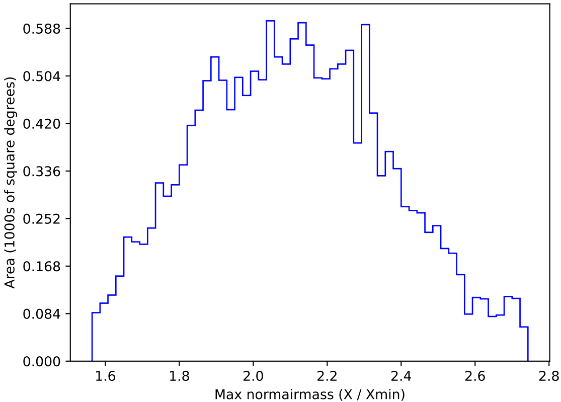
too_elab_r8_d3_giz_v3.4_10yrs WFD y band: Max normairmass
