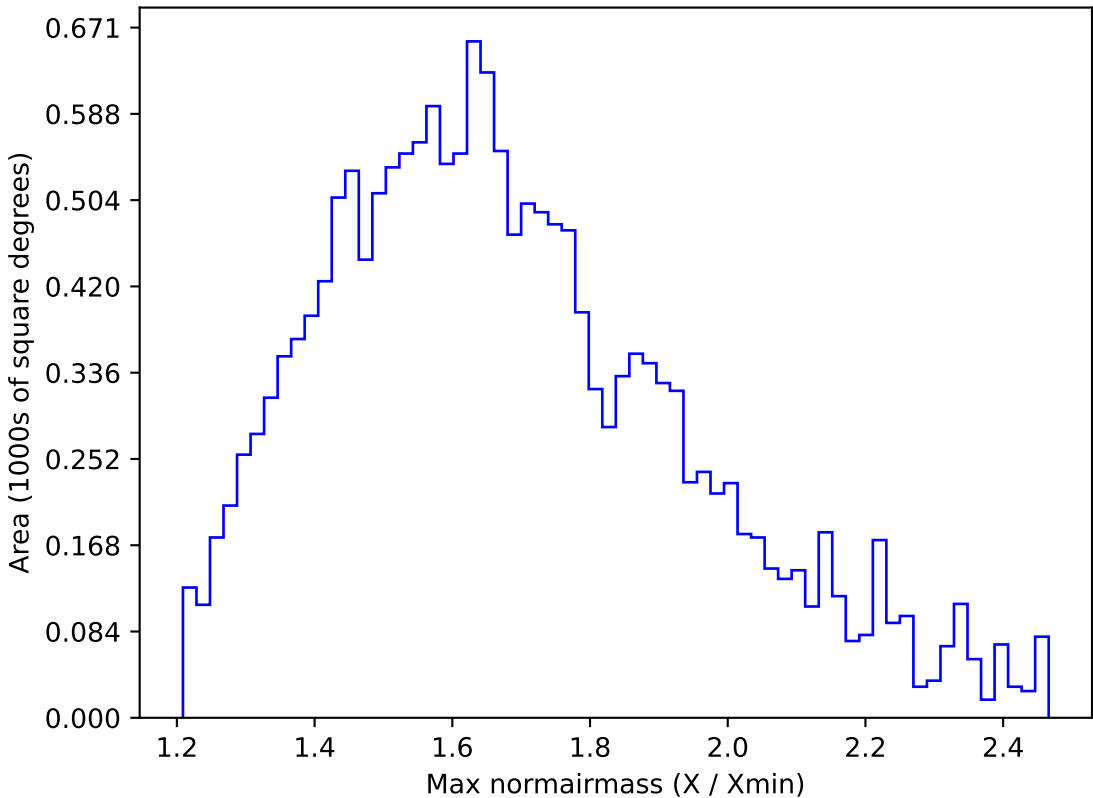
too_elab_r8_d3_giz_v3.4_10yrs WFD u band: Max normairmass
