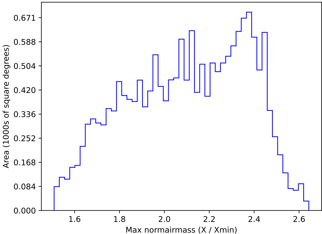
too_elab_r8_d3_giz_v3.4_10yrs WFD r band: Max normairmass
