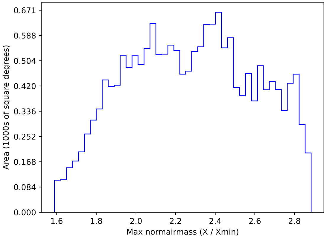
too_elab_r8_d3_giz_v3.4_10yrs WFD i band: Max normairmass
