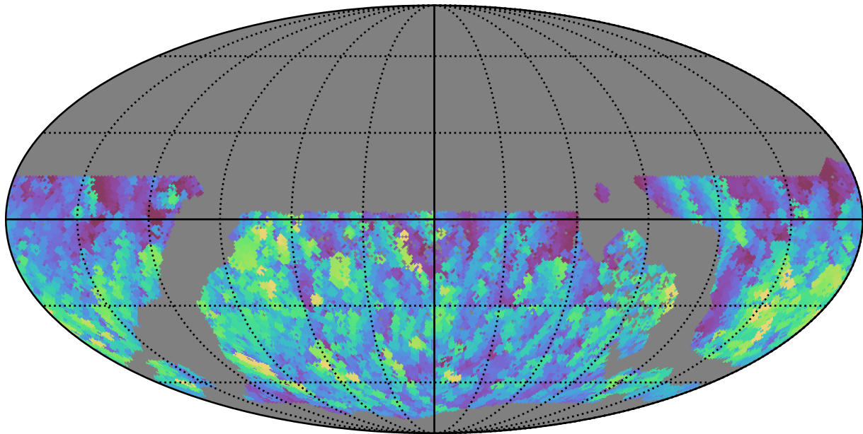
too_elab_r8_d3_giz_v3.4_10yrs WFD g band: Max normairmass
