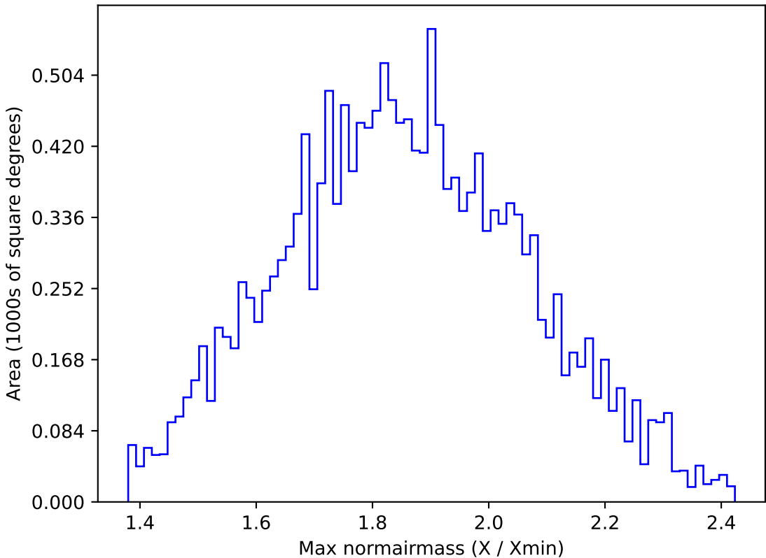
too_elab_r8_d3_giz_v3.4_10yrs WFD g band: Max normairmass
