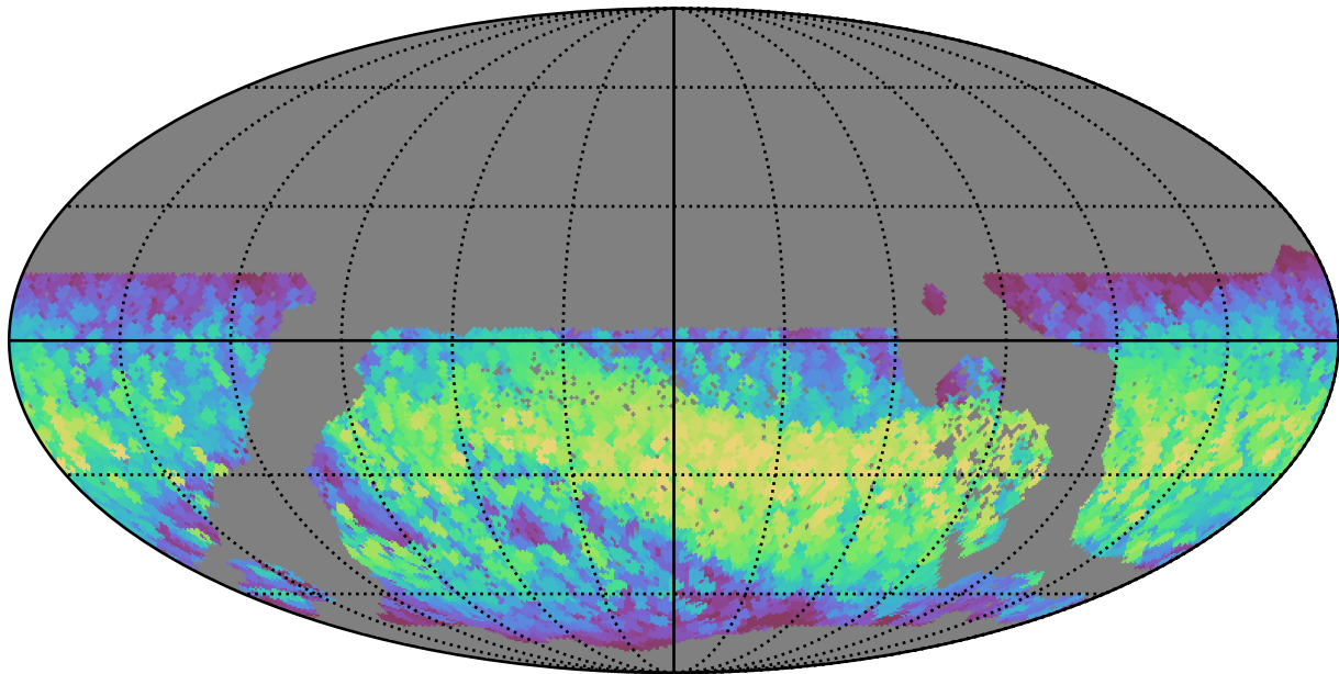
too_elab_r8_d3_giz_v3.4_10yrs WFD all bands: Max normairmass
