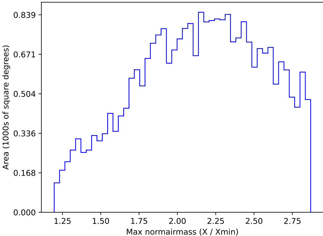
too_elab_r8_d3_giz_v3.4_10yrs All sky z band: Max normairmass
