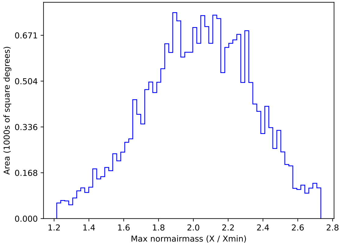
too_elab_r8_d3_giz_v3.4_10yrs All sky y band: Max normairmass
