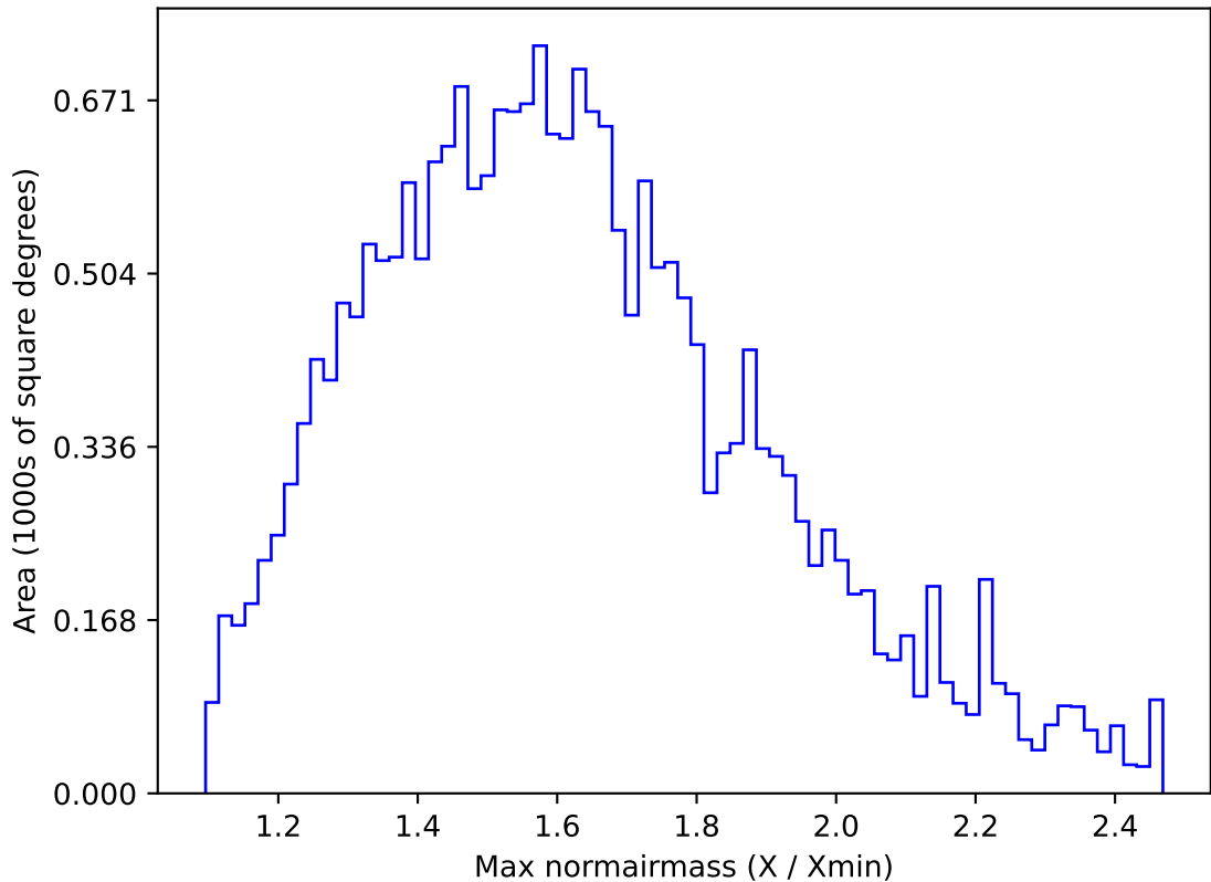
too_elab_r8_d3_giz_v3.4_10yrs All sky u band: Max normairmass
