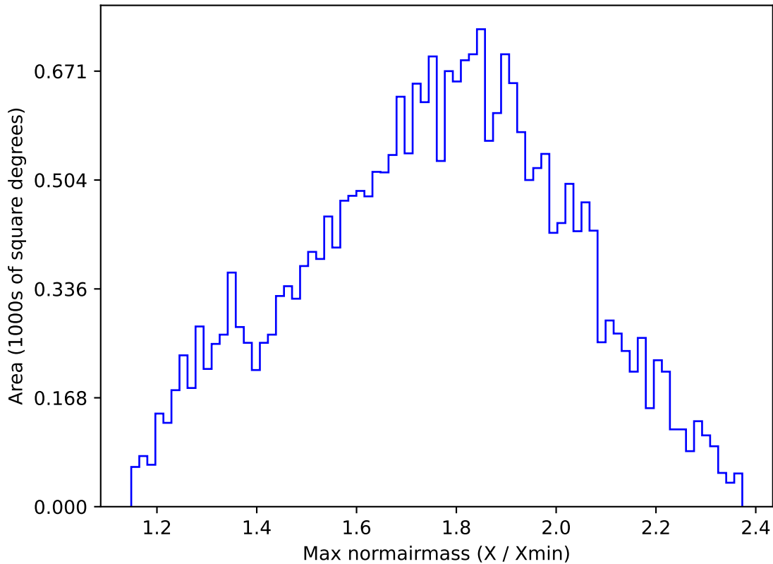
too_elab_r8_d3_giz_v3.4_10yrs All sky g band: Max normairmass
