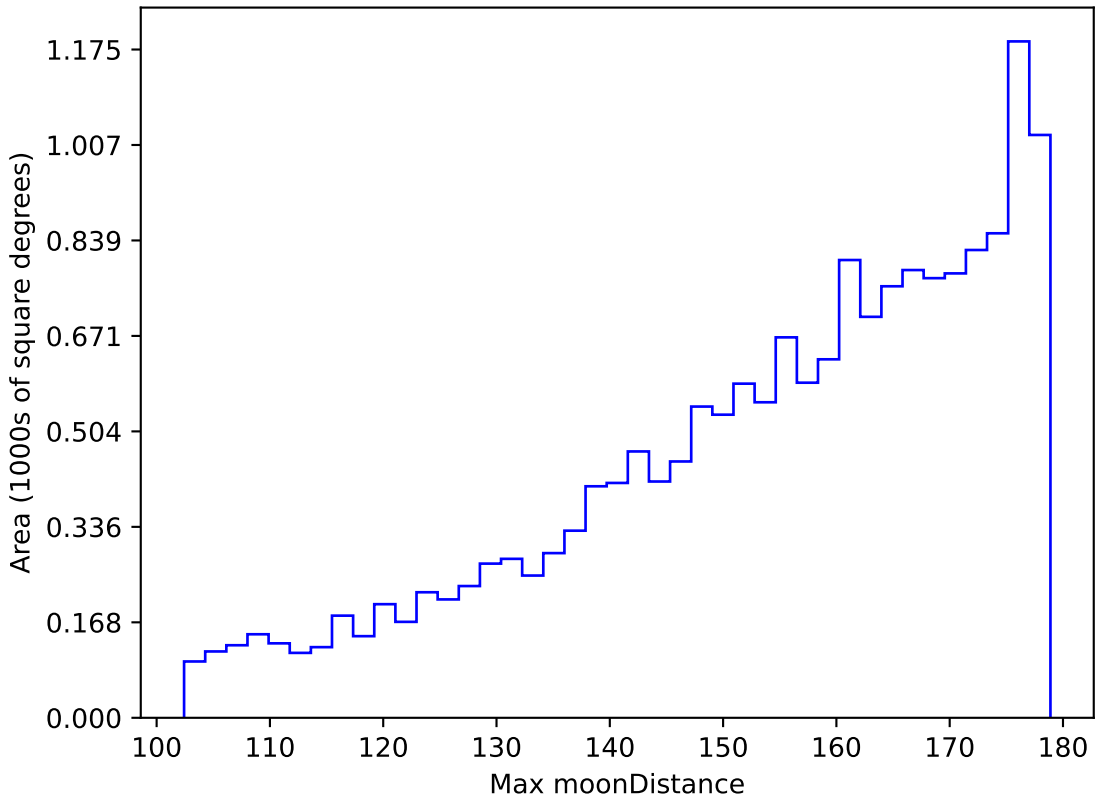
too_elab_r8_d3_giz_v3.4_10yrs WFD z band: Max moonDistance
