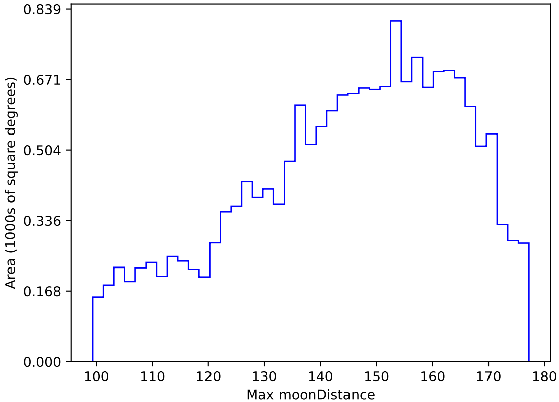
too_elab_r8_d3_giz_v3.4_10yrs WFD y band: Max moonDistance
