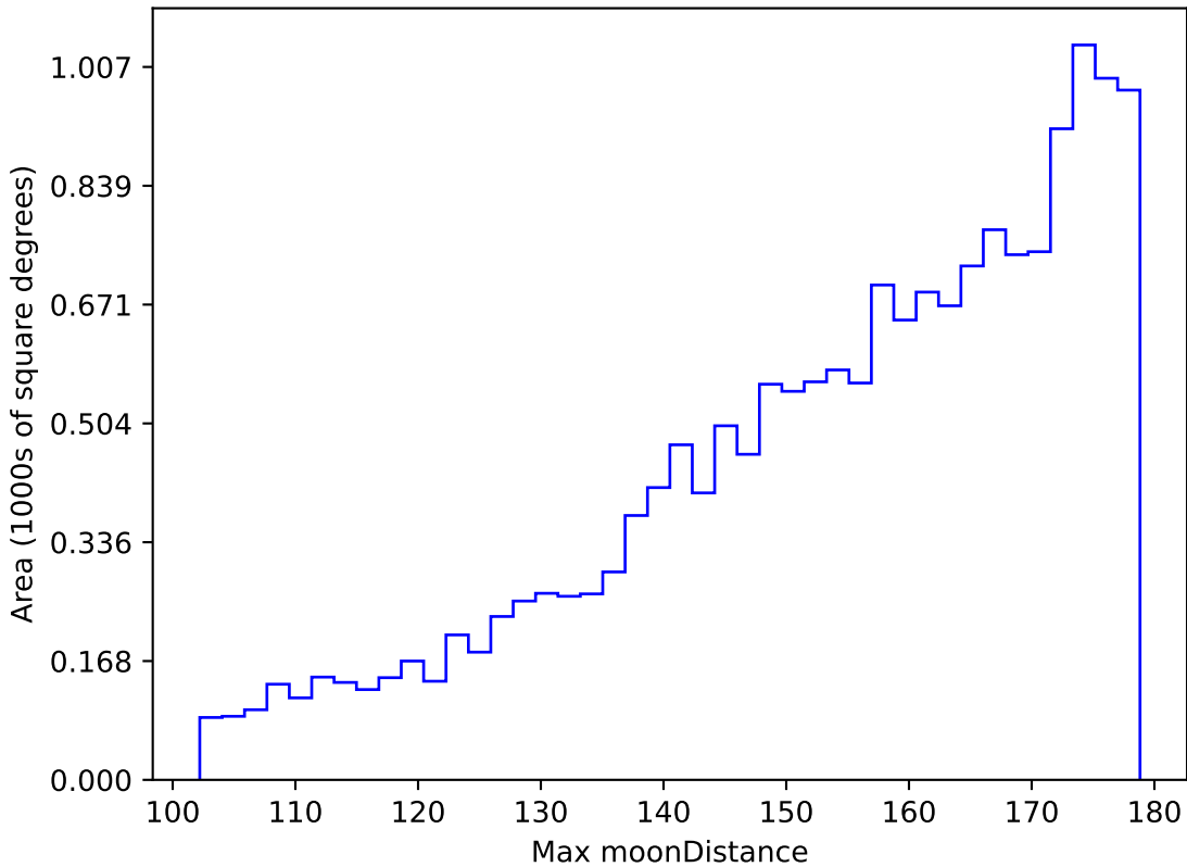
too_elab_r8_d3_giz_v3.4_10yrs WFD u band: Max moonDistance
