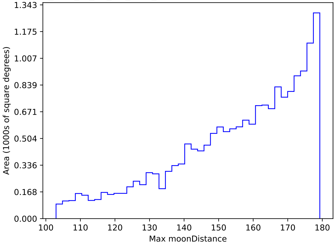
too_elab_r8_d3_giz_v3.4_10yrs WFD i band: Max moonDistance
