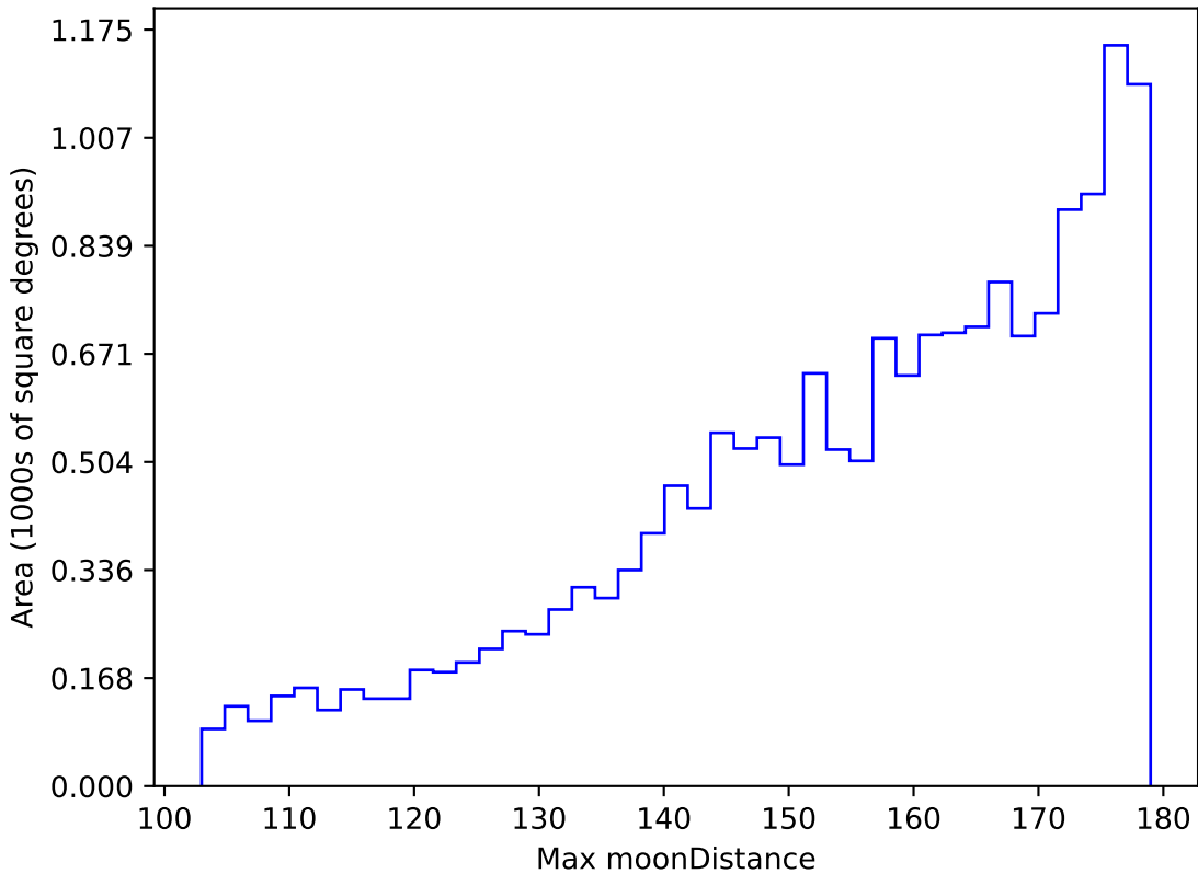
too_elab_r8_d3_giz_v3.4_10yrs WFD g band: Max moonDistance
