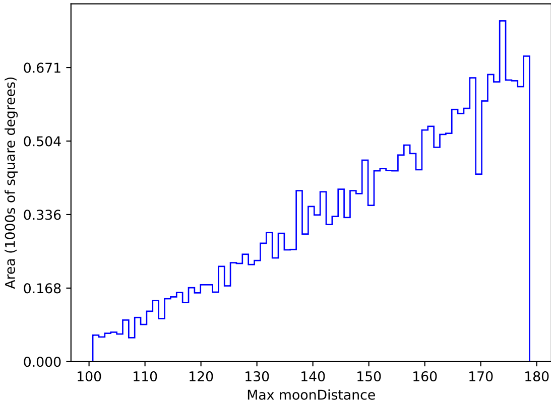
too_elab_r8_d3_giz_v3.4_10yrs All sky u band: Max moonDistance
