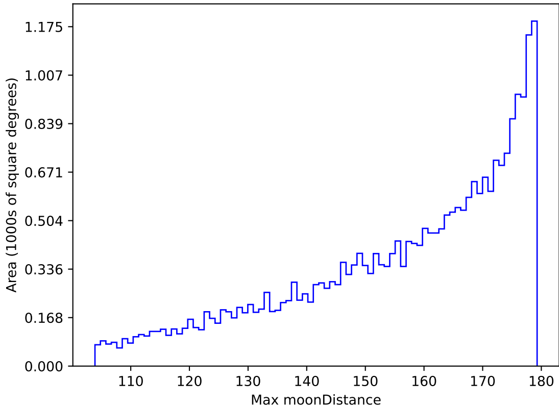
too_elab_r8_d3_giz_v3.4_10yrs All sky r band: Max moonDistance
